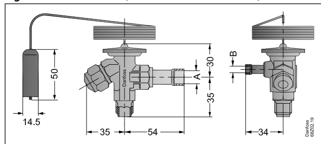
Figure 3: Flare × solder (All dimintions are in mm)
